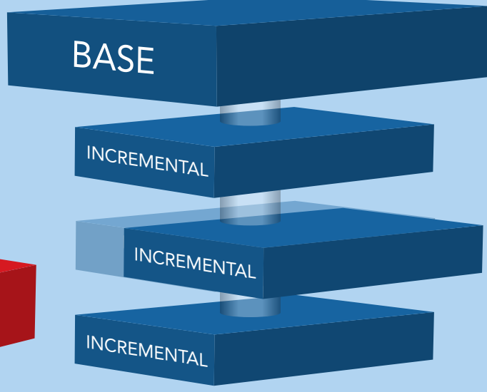
Datto's Inverse Chain
